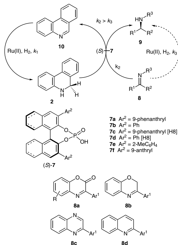
Scheme 6 Biomimetic asymmetric hydrogenation of 8 using a catalytic amount of phenanthridine ( 10 )
